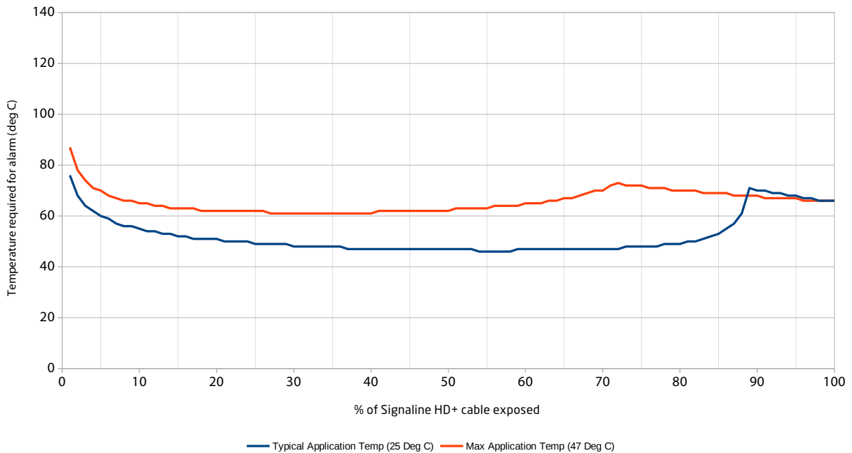
Chart A2 - Expected temperature required for an alarm in relation to percentage of Signaline HD+ LHD Cable in 64°C Setting
