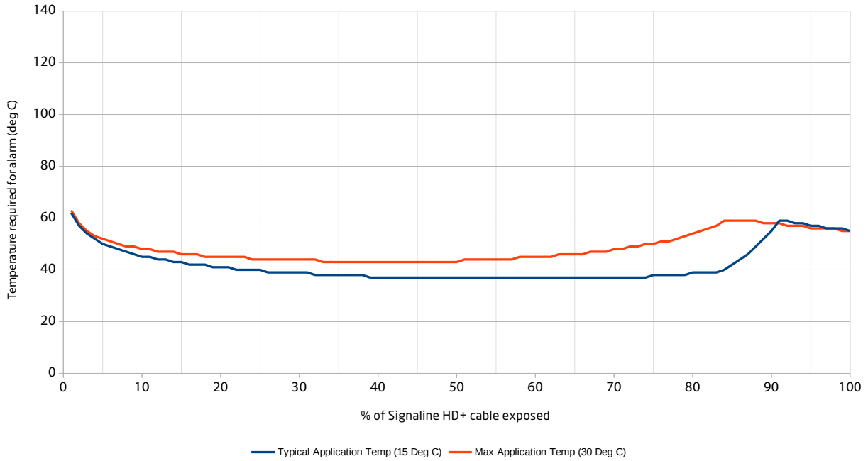
Chart A1 - Expected temperature required for an alarm in relation to percentage of Signaline HD+ LHD Cable in 54°C Setting
